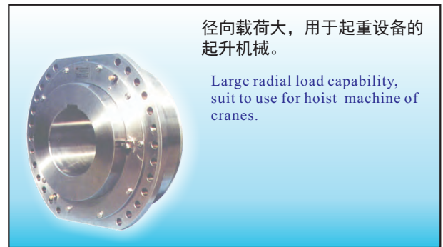
DC系列卷筒用鼓形齿式联轴器 Series DC curved tooth drum coupling
