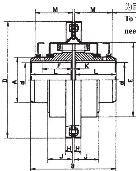
Construction dwg. of JS201~JS216
