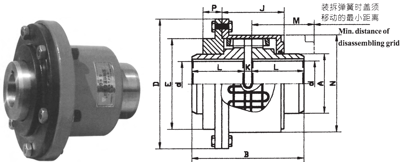
Construction dwg. of JS702~JS717
