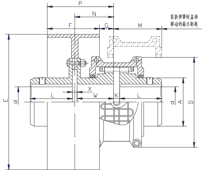
Construction dwg. of JS26205~JS6215
