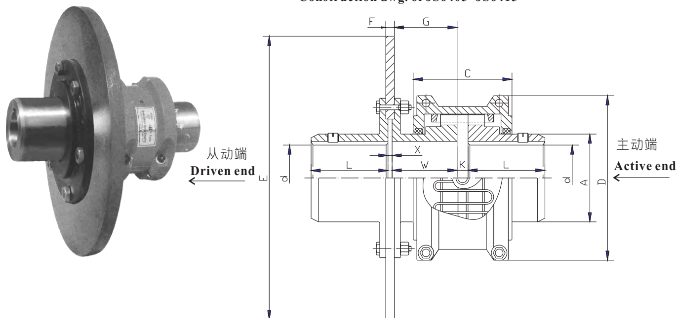
Construction dwg. of JS6405~JS6415
